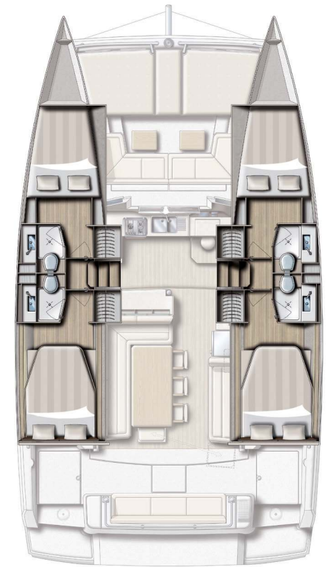
4 CABINS / 4 HEADS VERSION VERSION 4 CABINES / 4 SDB
